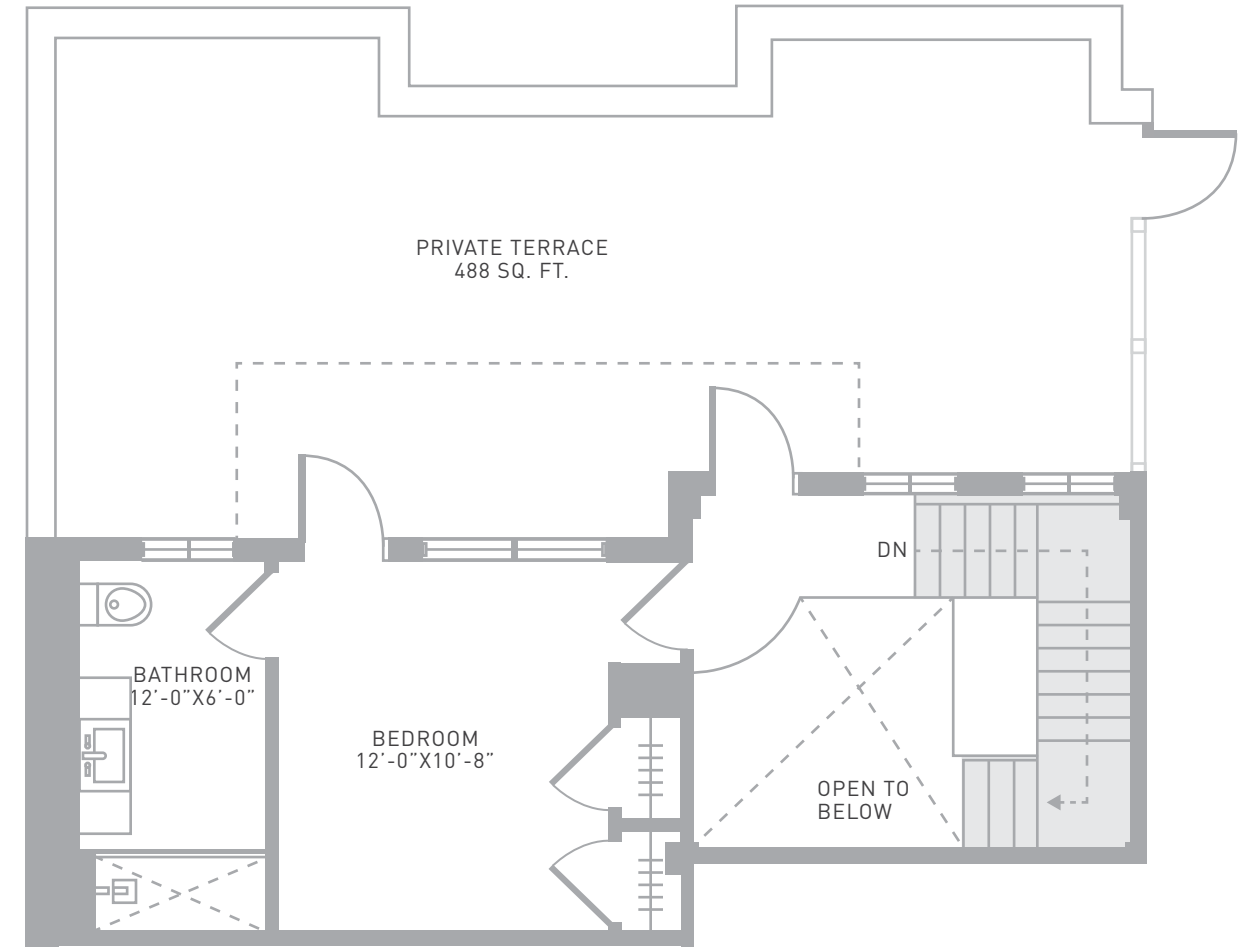
MEZZANINE
